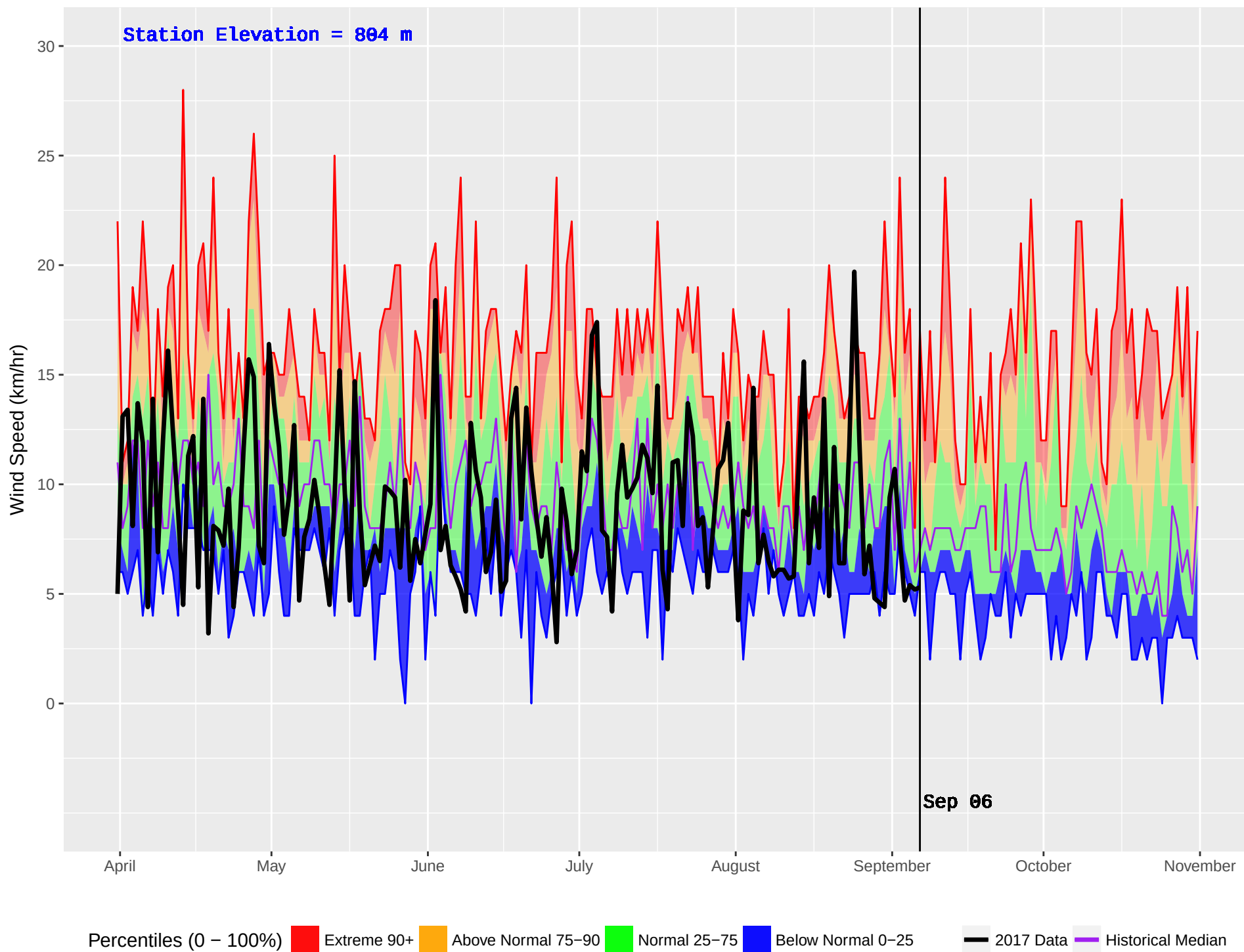
KOOCANUSA (1075) : Historical (2010–2016) and Current (2017) Noon Wind Speed
