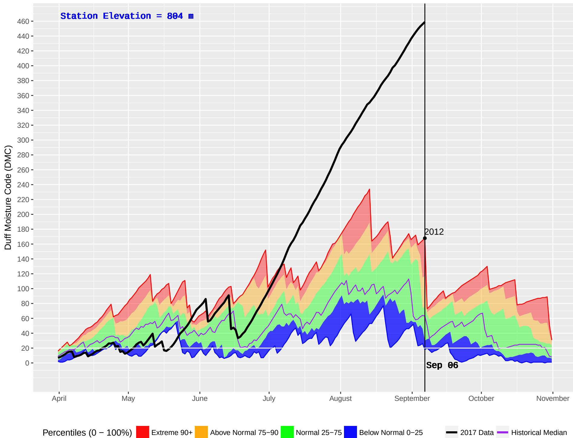
KOOCANUSA (1075) : Historical (2010–2016) and Current (2017) Noon Duff Moisture Code (DMC)
